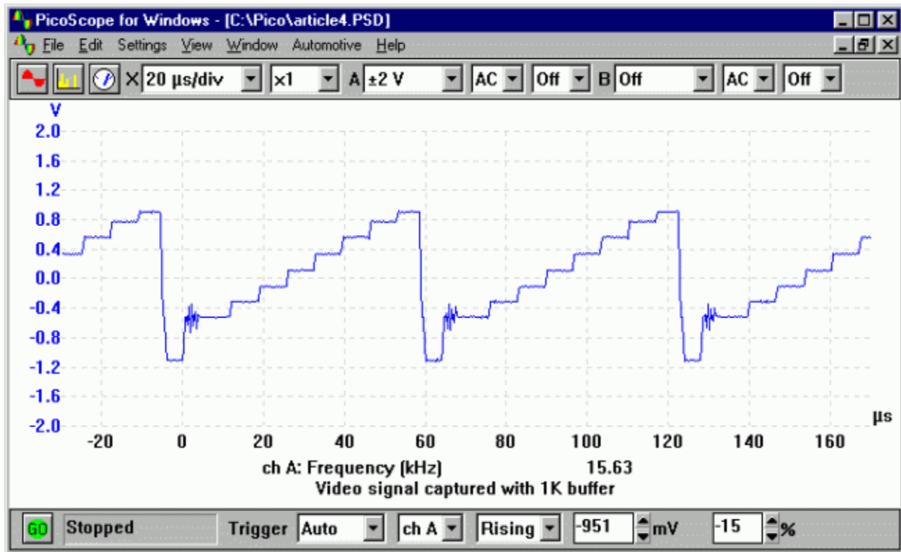
figure 2a: 200uS of a video wave captured with a 1K buffer memory.
