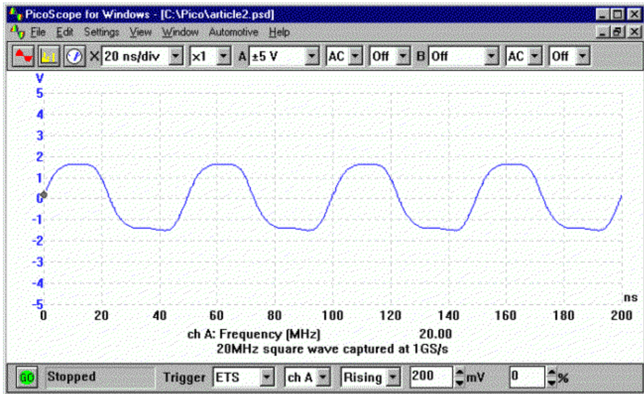
figure 1b: 20MHz square wave captured at 1GS/s.
